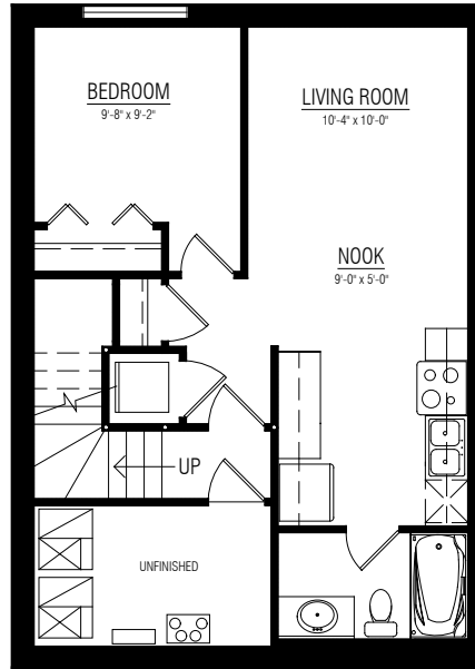
GALLEY KITCHEN OPTION - 544 SQ.FT.
